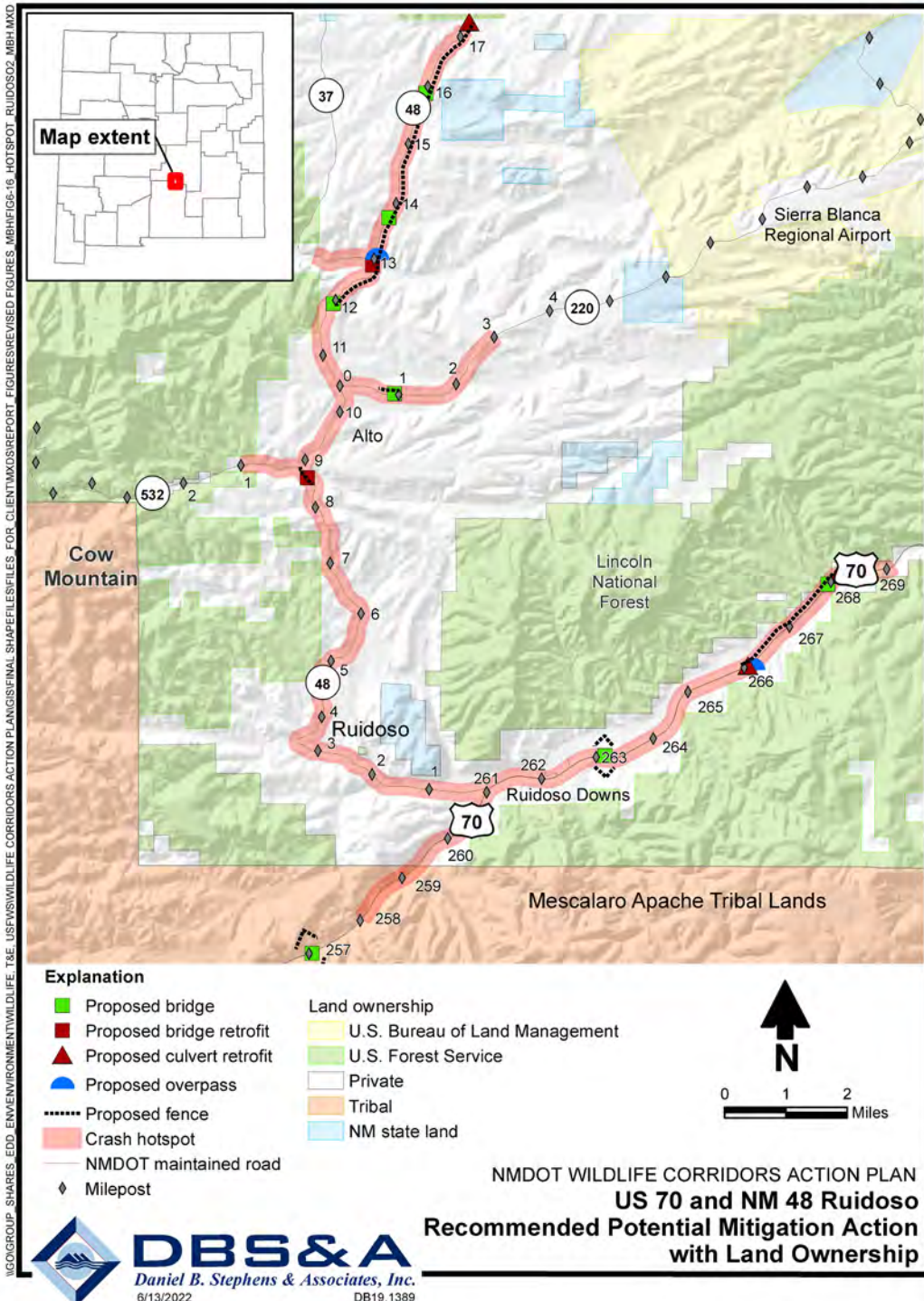
Figure 6-17. Land ownership and recommended project mitigation actions in US 70 and NM 48 Ruidoso hotspot.
