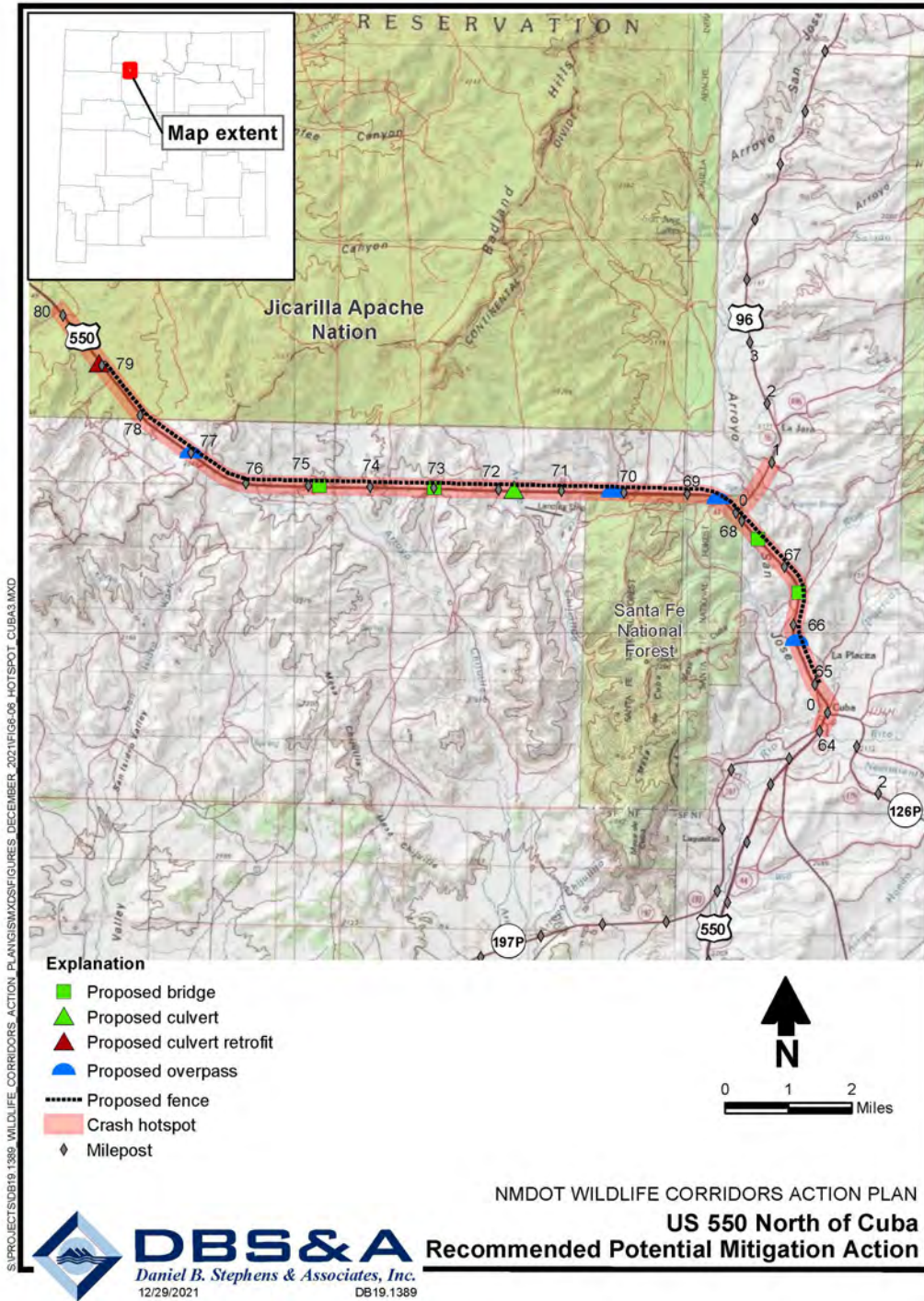
Figure 6-7. Top priority mitigation recommendations for the US 550 North of Cuba hotspot.
