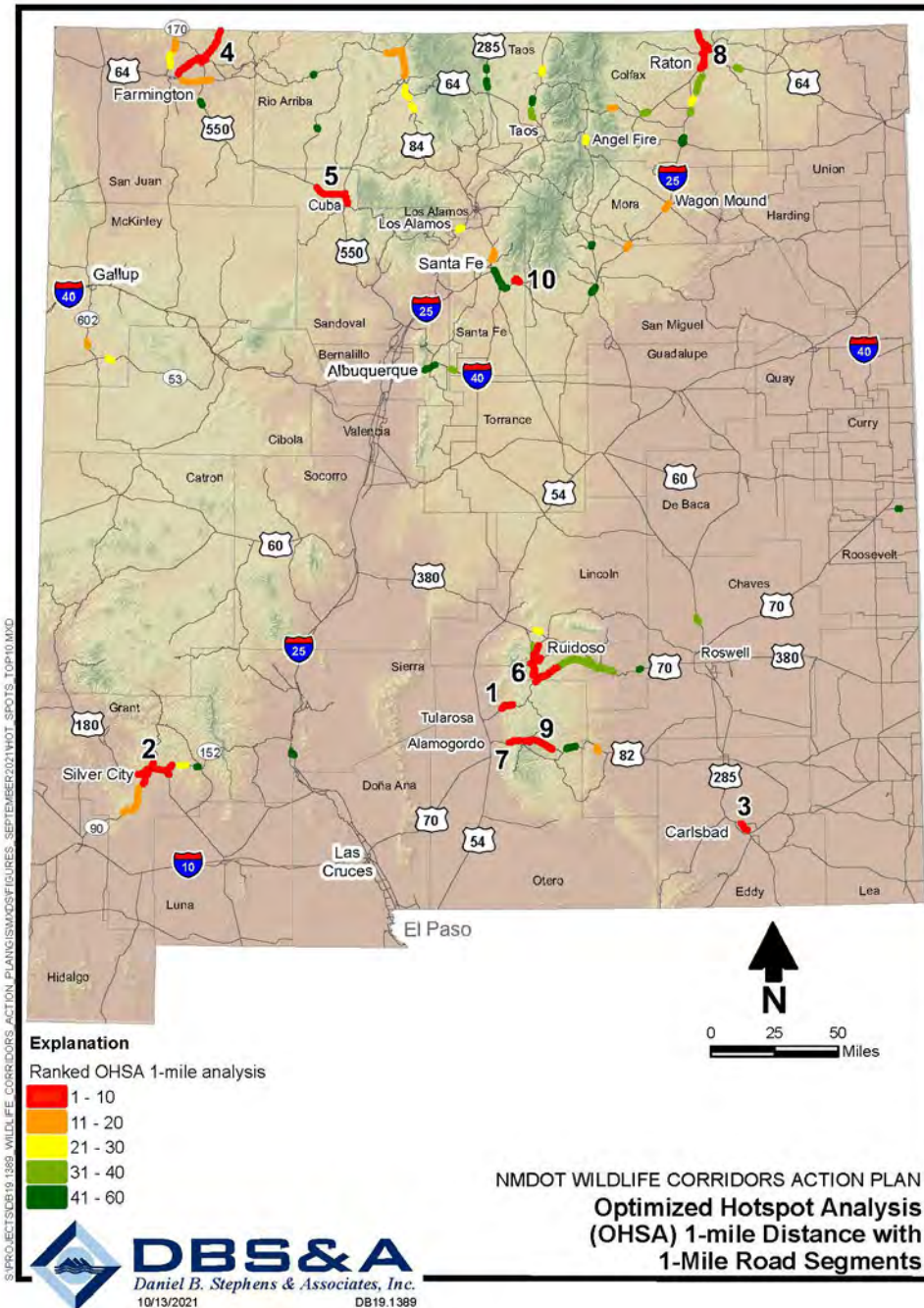
Figure ES-1. Hotspot analysis results. A total of 60 wildlife-vehicle crash hotspots were identified. Only the top 10 hotspots are numbered.
