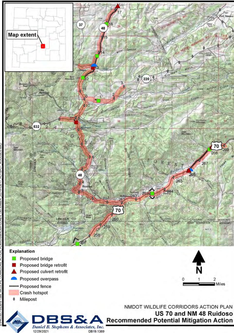
Figure 6-18. Top priority mitigation recommendations for US 70 and NM 88 Ruidoso hotspot.
