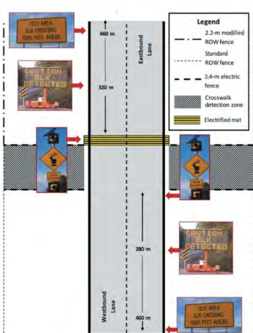
Figure D-54. Combination of signage used to successfully reduce speed and increase braking response of motorists along SR 260 in Arizona (from Gagnon et al., 2019).
