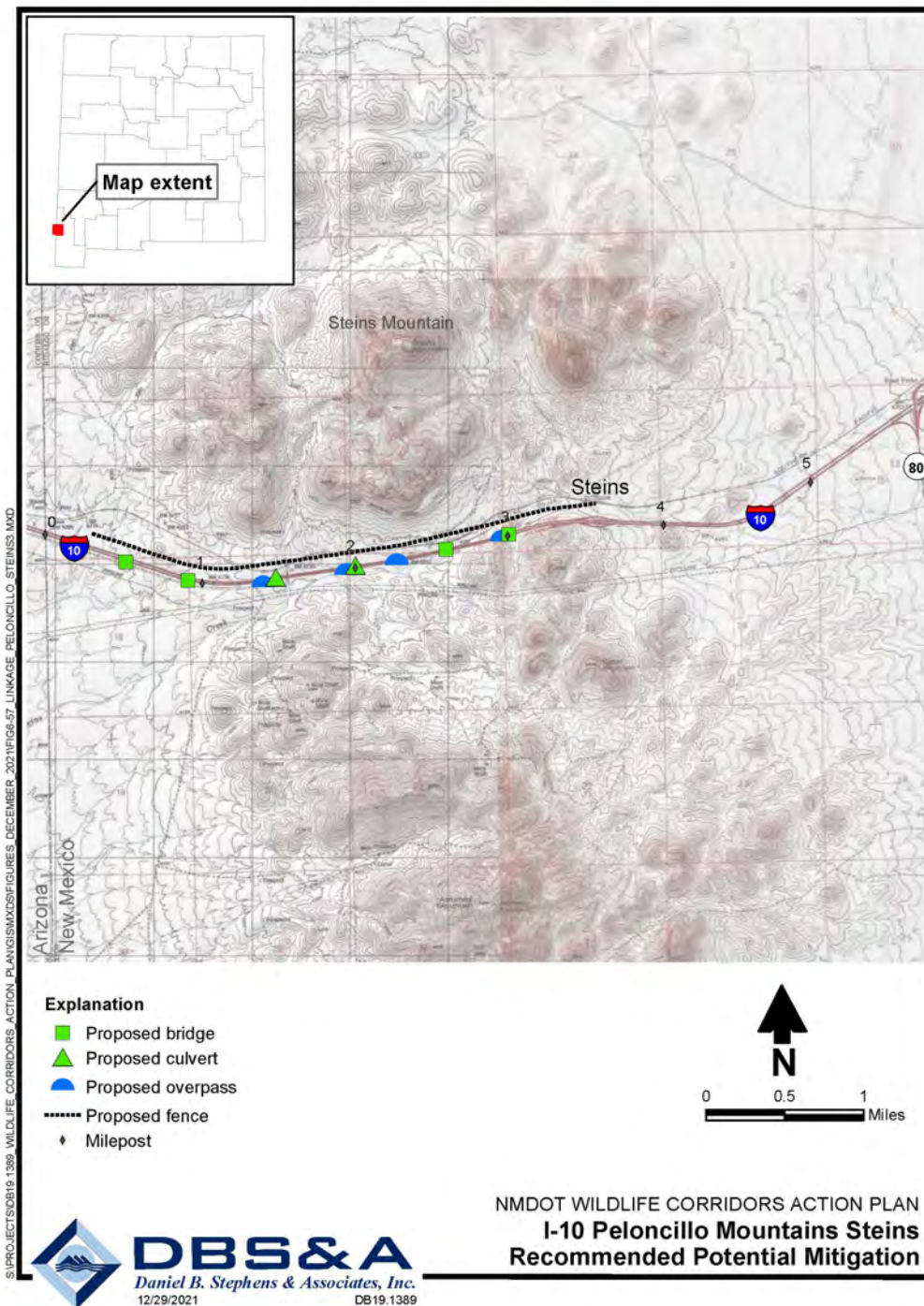
Figure 6-58. Top priority mitigation recommendations for the Peloncillo Mountains wildlife corridor.
