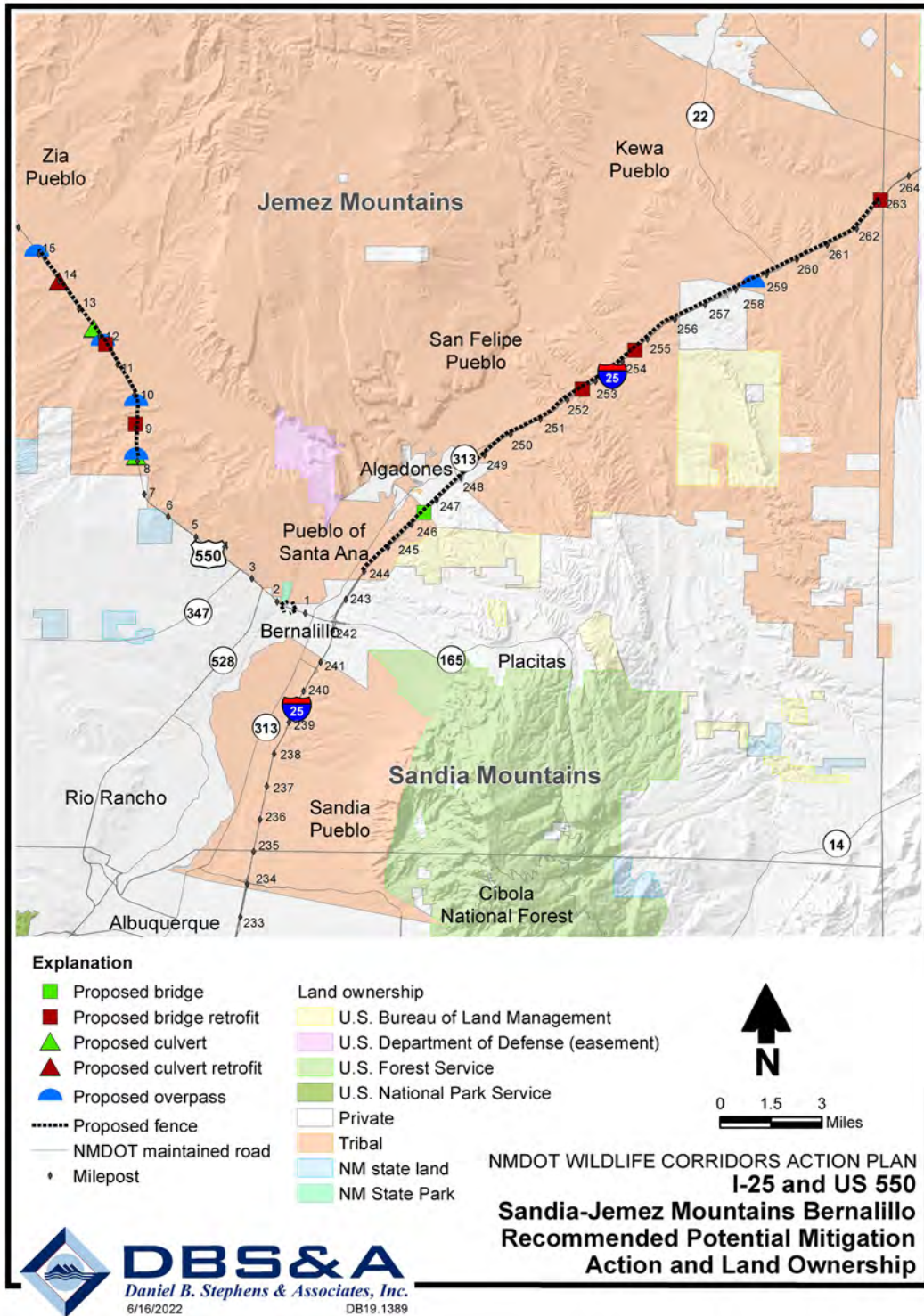
Figure 6-69. Land ownership and recommended project mitigation actions in the Sandia-Jemez Mountains wildlife corridor.
