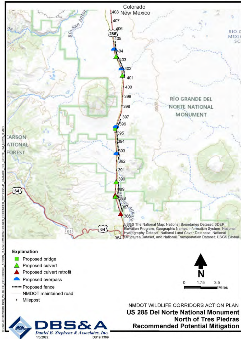
Figure 6-42. Top priority mitigation recommendations for the Del Norte wildlife corridor.
