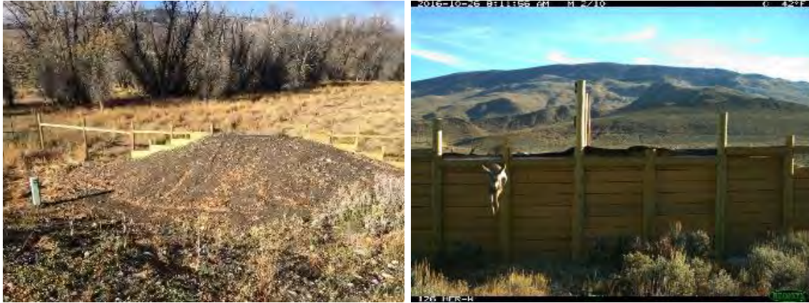
Figure D-36. Colorado SH 9 most successful escape ramp type with a 3:1 slope and no center fence (left) (photo credit: P. Cramer). Mule deer using escape ramp with center fence in Colorado, SR 9 (right) (photo credit: CDOT, CPW, Eco-Resolutions).
