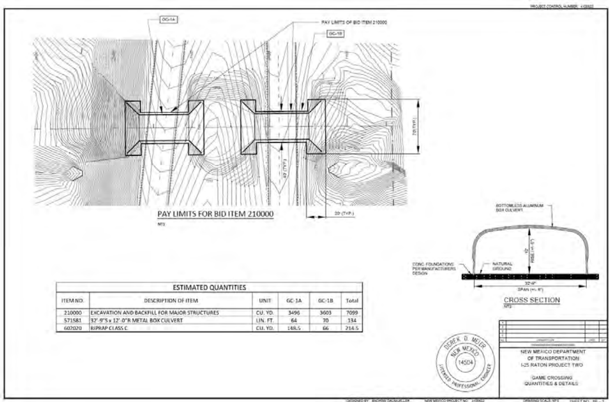
Figure A-10. I-25 Raton Pass plans for wildlife crossing metal arch culverts.
