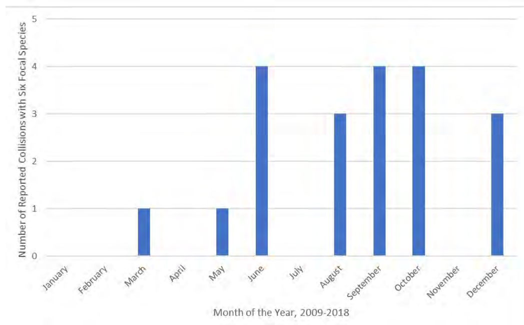
Figure 6-62. NMDOT wildlife-vehicle crash data by month in Sandia-Jemez Mountains wildlife corridor.
