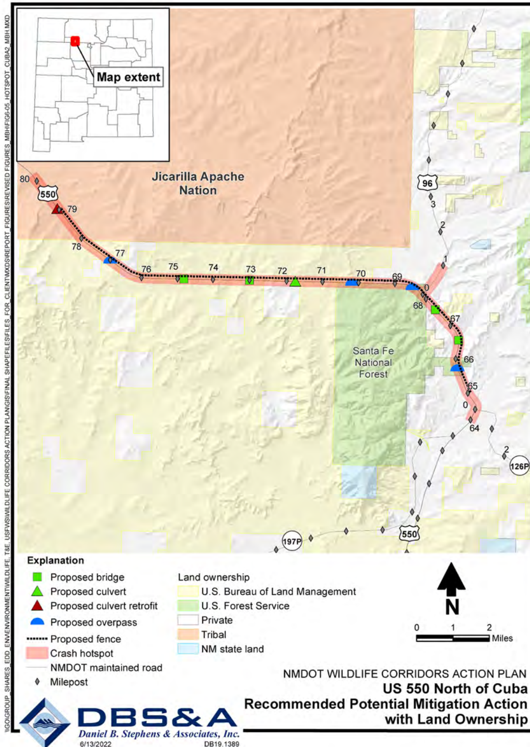
Figure 6-6. Land ownership and recommended project mitigation actions in the US 550 North of Cuba hotspot.
