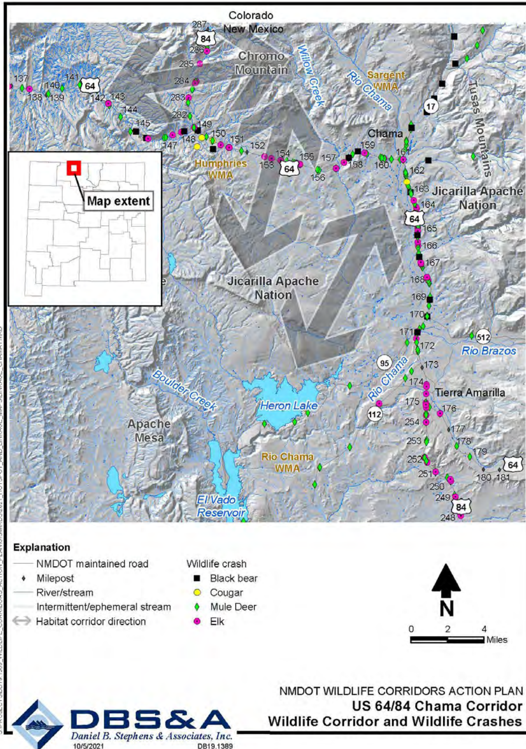
Figure 6-31. Wildlife-vehicle crashes (2009–2018) and wildlife movement in the Chama wildlife corridor.
