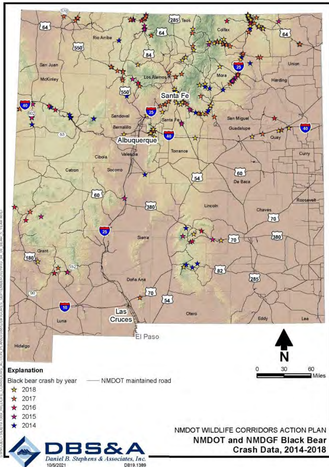
Figure 4-8. Reported crashes with black bear, 2014-2018.
